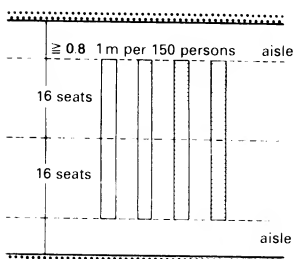
③ Row width: 16 seats
